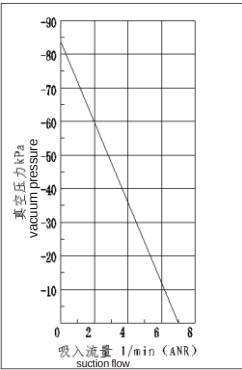
流量特性:flow characteristic
